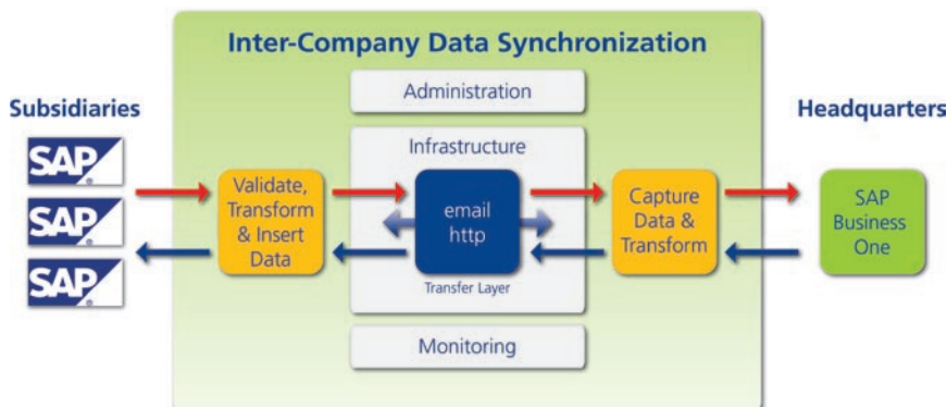
iBOLT Inter-Company Data Synchronization Accelerator's Architecture in a Typical Business Scenario
